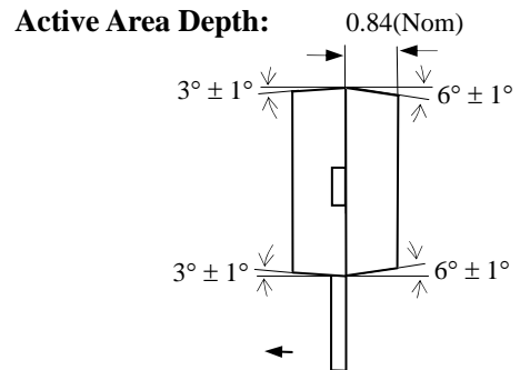
Sensor Location
